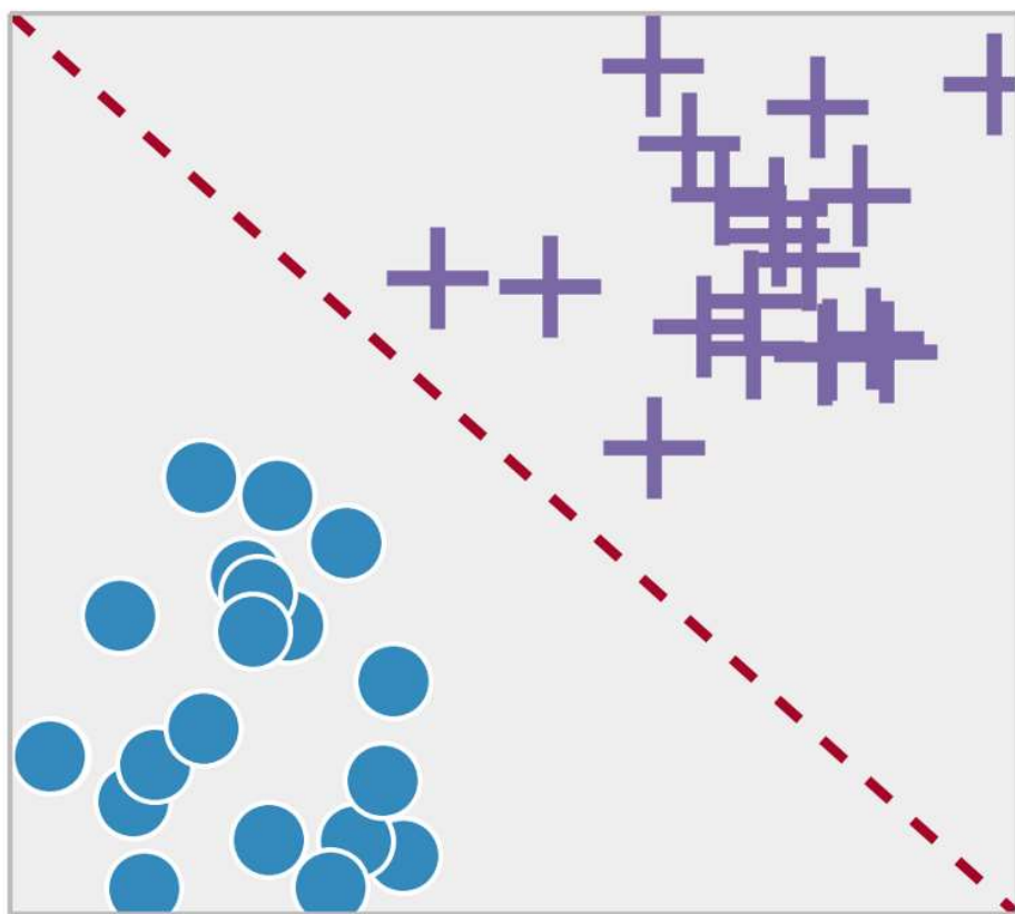
Classification
