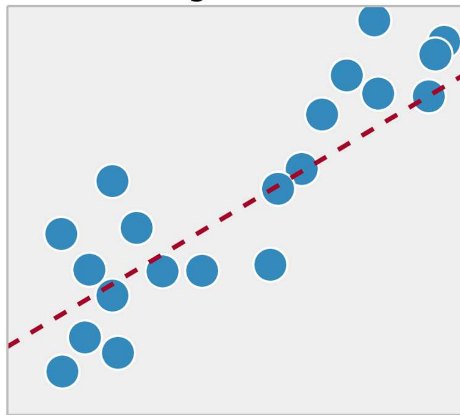
Regression
