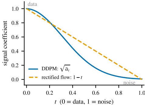
Figure 1: The diffusion path and the rectified-flow path between data and noise. The flow objective regresses a constant velocity along a straight line; the diffusion objective traverses a curved, non-uniform-speed path.
