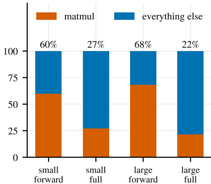
(b) matmul share of kernel time
