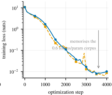
(b) training loss collapses
