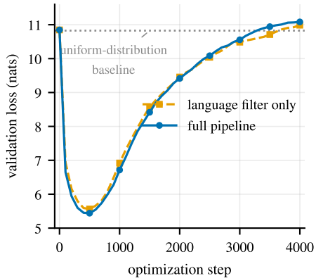
(a) validation loss degrades
