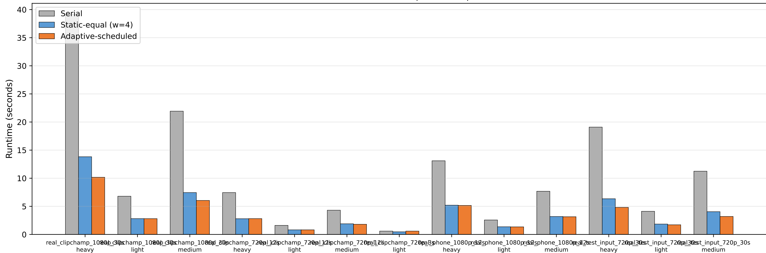
Execution Time: Serial vs Static-Equal vs Adaptive-Scheduled
