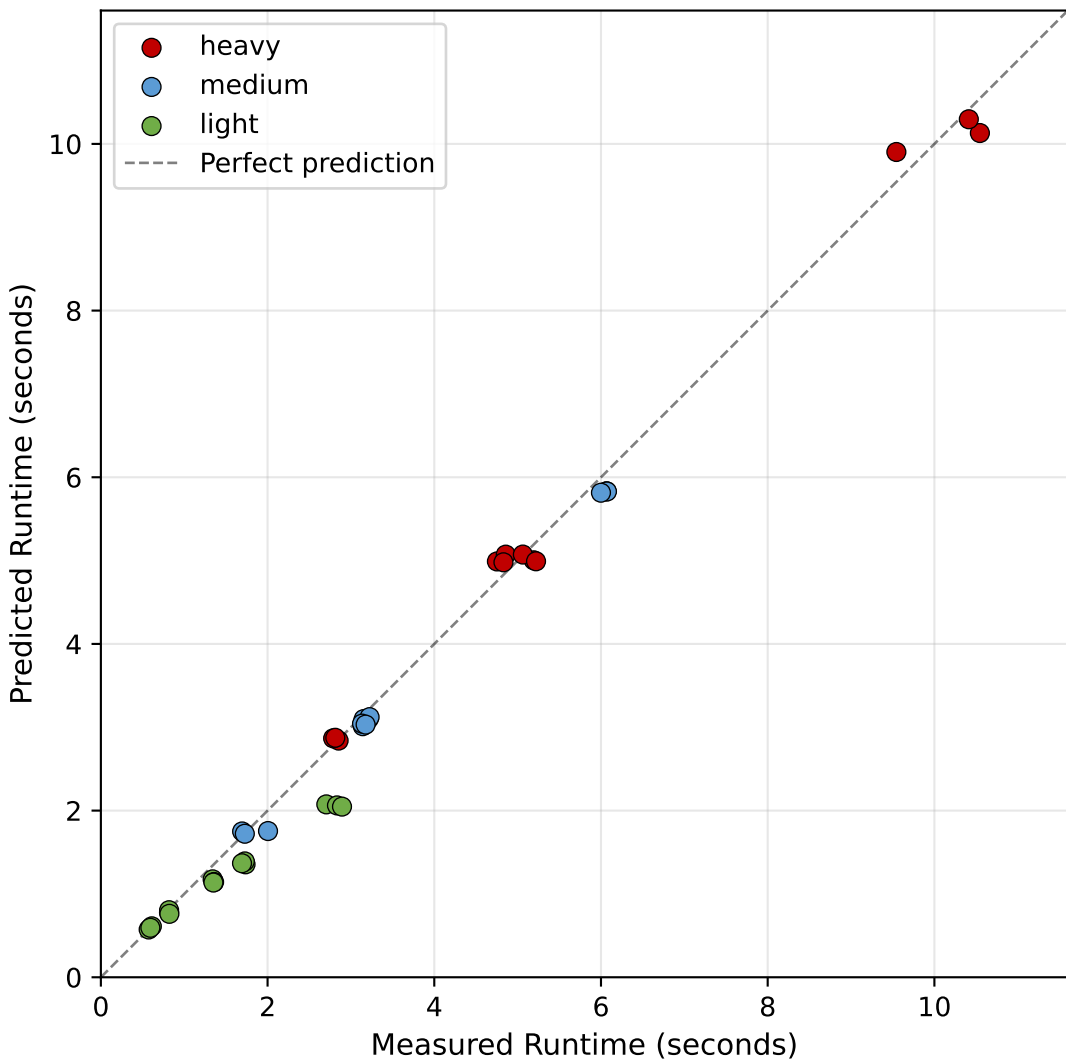
Cost Model Calibration: Predicted vs Measured
