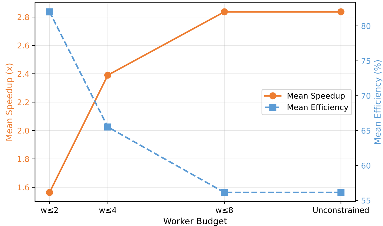
Resource-Budgeted Selection: Speedup vs Efficiency
