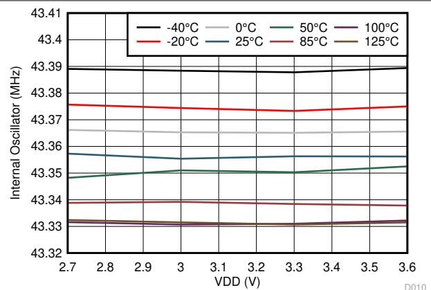
Figure 6-9. Internal Oscillator Frequency vs VDD
