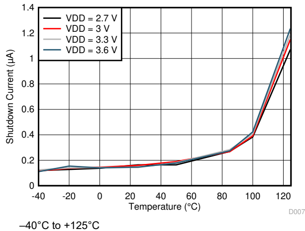
Figure 6-6. Shutdown Mode IDD vs Temperature
