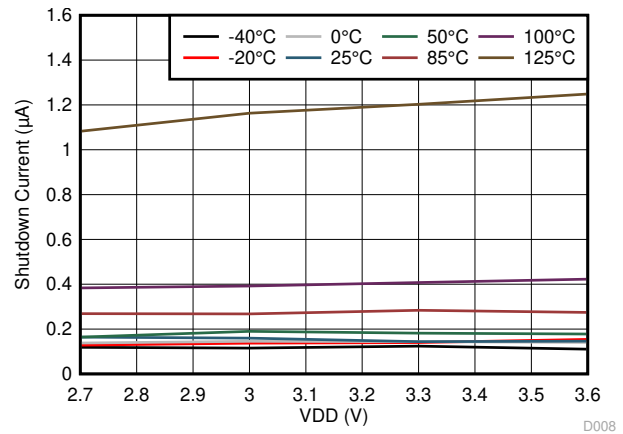
Figure 6-7. Shutdown Mode IDD vs VDD
