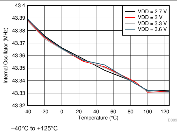
Figure 6-8. Internal Oscillator Frequency vs Temperature
