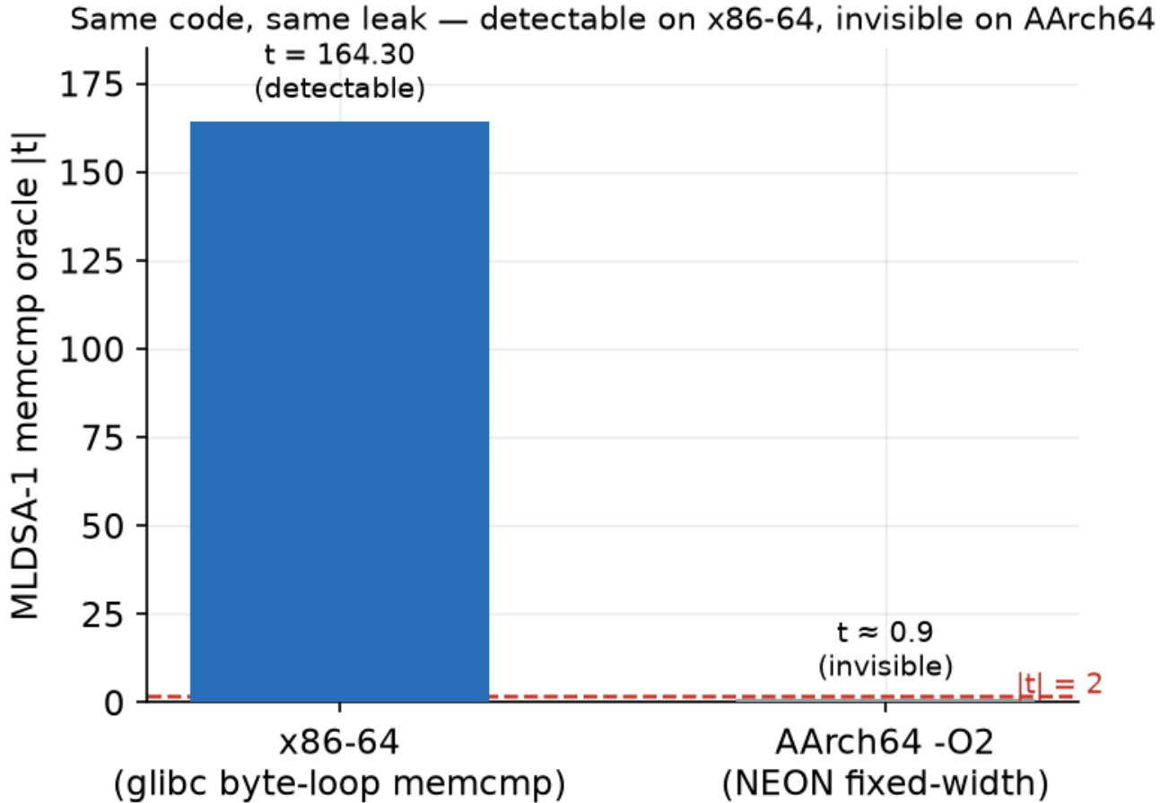
Figure 4. ISA portability of the ML-DISA-44 memcmp oracle. The identical source leaks measurably on x86-64 (glibc byte-loop memcmp, t=164.30 ) but is invisible on AArch64 at -O2, where the 32-byte comparison compiles to fixed-width NEON instructions with no per-byte early exit ( t \approx 0.9 ). A timing audit run only on ARM hardware would miss this leak entirely.
