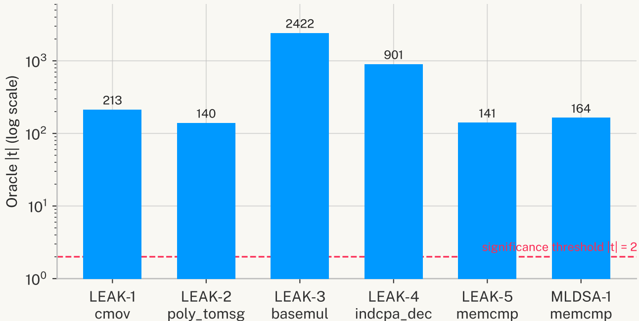
LLM-confirmed timing signal for every leak — AFL++ detected none (24 h, ~120M execs/target)
