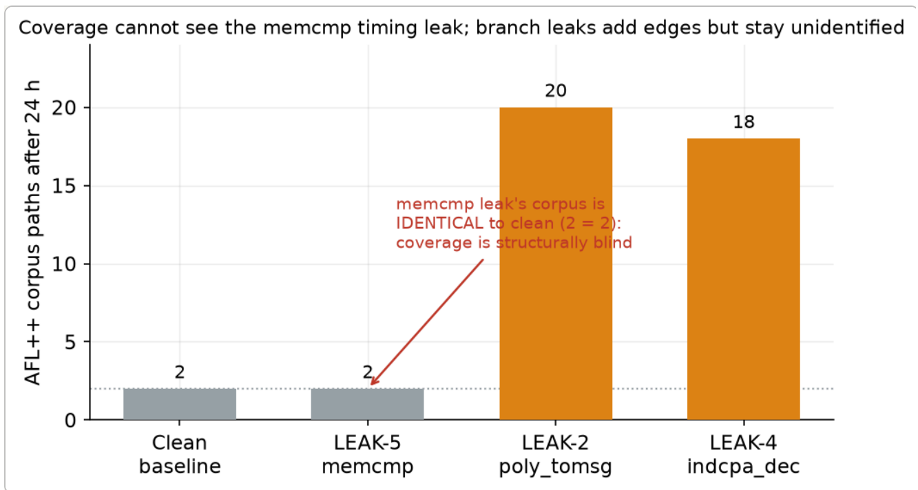
Figure 3. AFL++ corpus paths after 24 hours. The memcmp leak (LEAK-5) produces a corpus identical to the clean baseline (2 = 2) – coverage-guided fuzzing cannot distinguish the weakened implementation from the correct one. Branch leaks (LEAK-2/4) add coverage edges, but AFL++ still cannot identify them as timing-sensitive.
