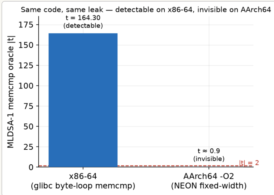
Figure 4. ISA portability of the ML-Dsa-44 memcmp oracle. The identical source leaks measurably on x86-64 (glibc byte-loop memcmp, t=164.30 ) but is invisible on AArch64 at -O2, where the 32-byte comparison compiles to fixed-width NEON instructions with no per-byte early exit ( t \approx 0.9 ). A timing audit run only on ARM hardware would miss this leak entirely.
