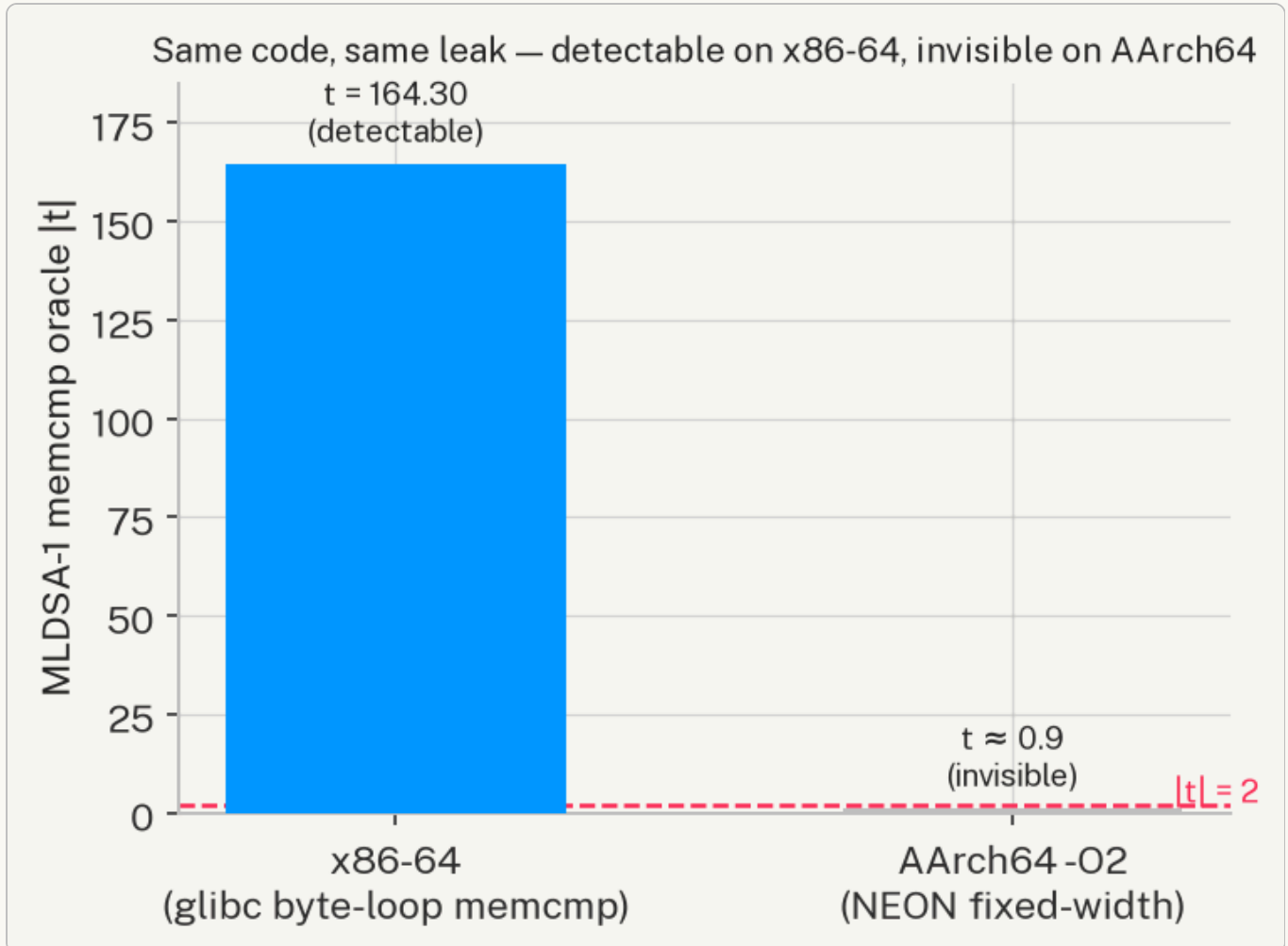
Figure 4. ISA portability of the ML-DISA-44 memcmp oracle. The identical source leaks measurably on x86-64 (glibc byte-loop memcmp , t=164.30 ) but is invisible on AArch64 at -O2, where the 32-byte comparison compiles to fixed-width NEON instructions with no per-byte early exit ( t \approx 0.9 ). A timing audit run only on ARM hardware would miss this leak entirely.
