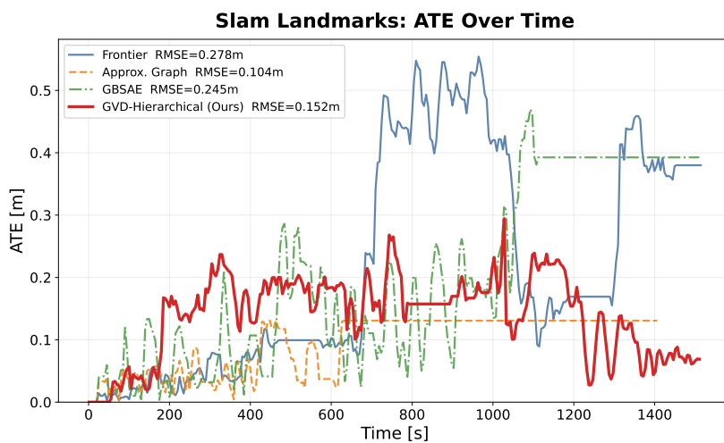
Fig. 4. ATE over time on the slam_landmarks map.
