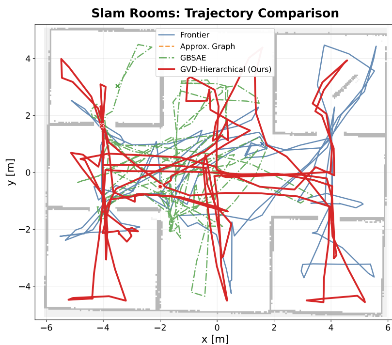
Fig. 3. Trajectory comparison on the complex slam_rooms map.
