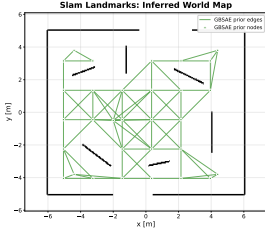
(a) slam_landmarks
