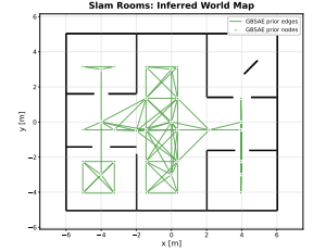
(c) slam_rooms
