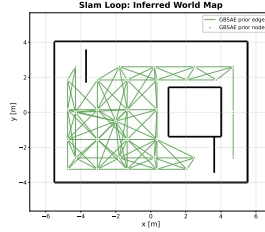
(b) slam_loop
