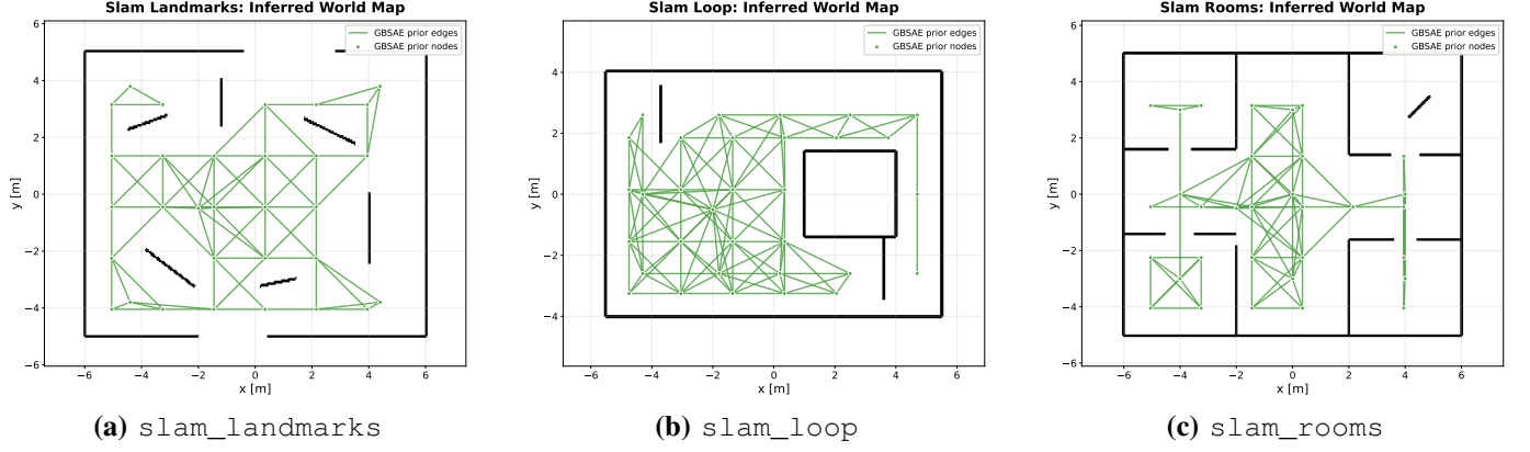
Fig. 1. Simulation maps used for evaluating active exploration policies. The green overlay denotes the prior graph used by GBSAE.
