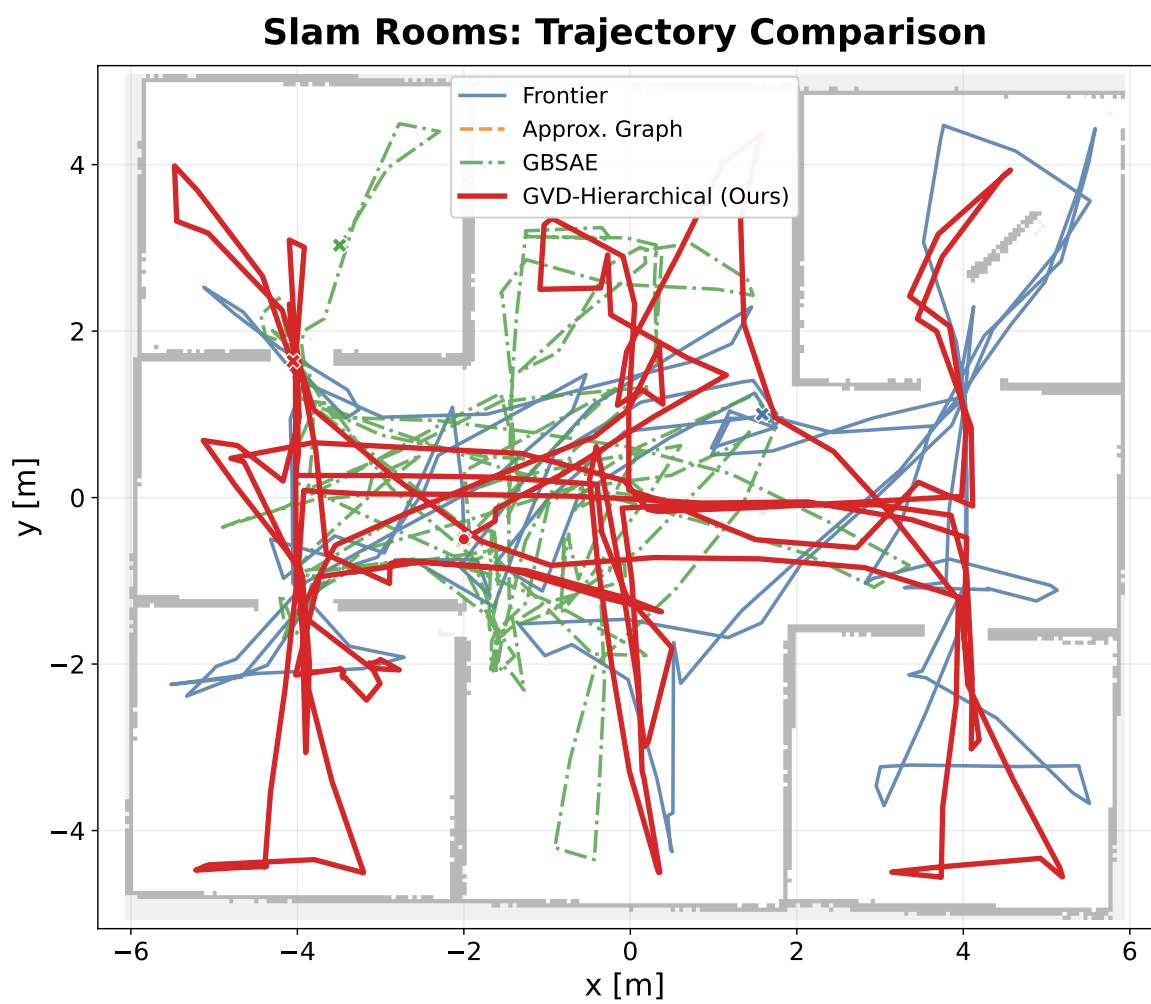
Fig. 3. Trajectory comparison on the complex slam_rooms map.
