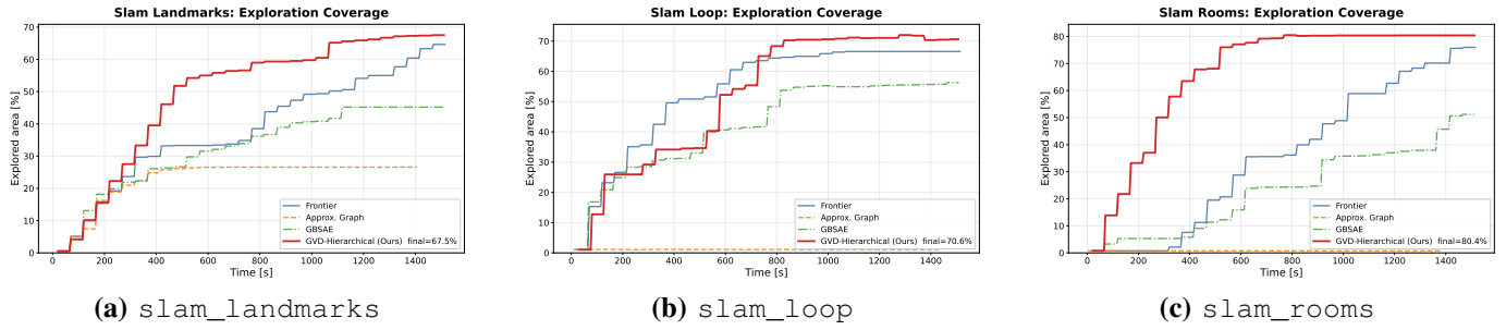
Fig. 2. Coverage growth comparison across the three simulation maps.
