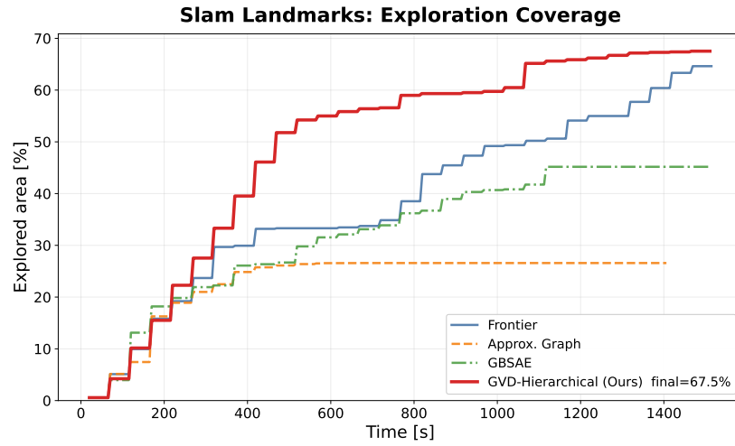
(a) slam_landmarks
