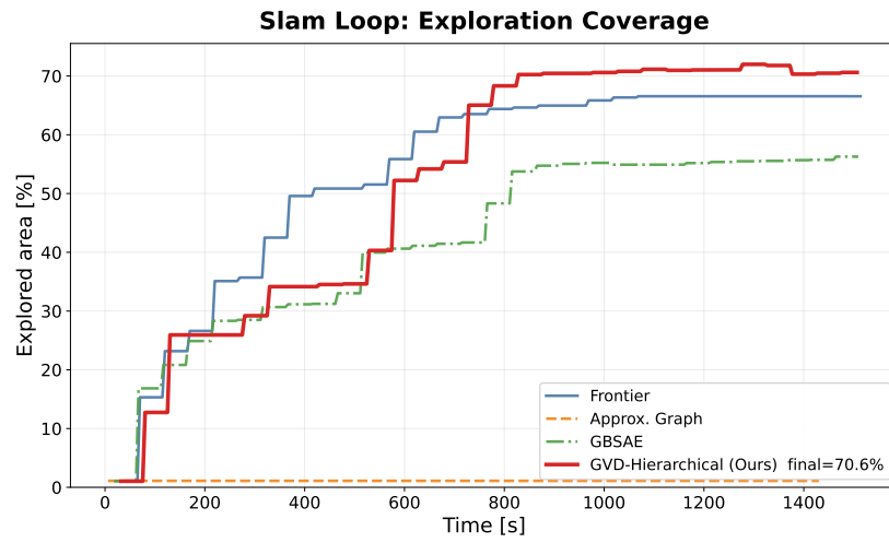
(b) slam_loop
