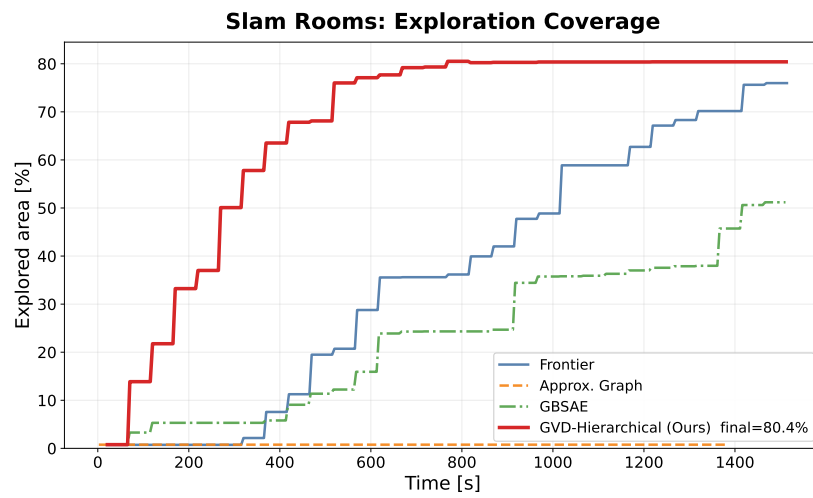
(c) slam_rooms
