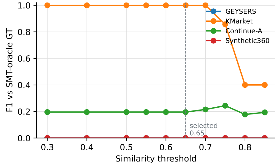
(a) F1 across thresholds
