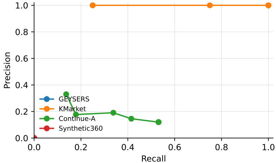
(b) Precision-recall trace
