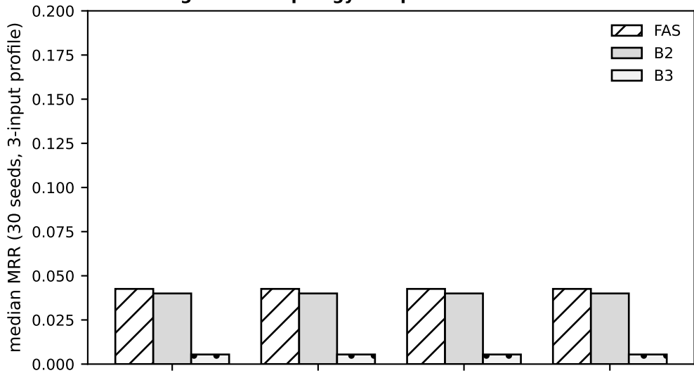
Figure 7. Four topologies (300 nodes, 3 inputs, 300 distractors, 50 % noise); topology type moves the absolute difficulty but never separates the mechanisms. B1 (direct 2-hop accumulation) is definitionally 0 here (no input \rightarrow joint edge); B3 random \approx chance.
