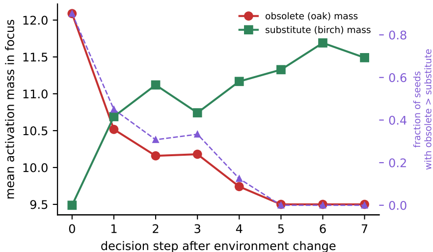
T3 re-routing: stale vs new context (n=20 seeds)
