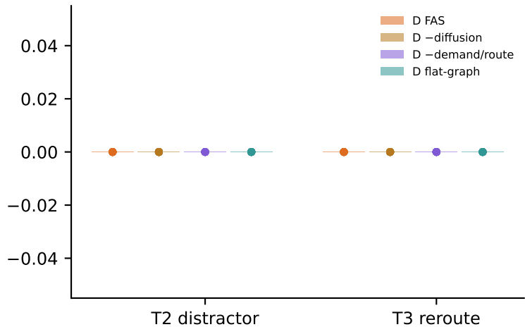
distractor rate
