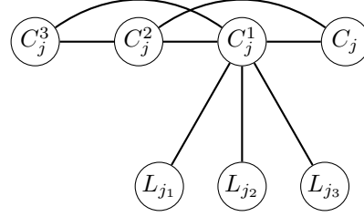
(iv) Literal-complement structure
