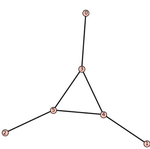
(a) The root graph G .
