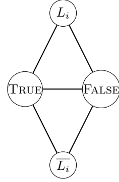
(iv) Literal-complement structure
