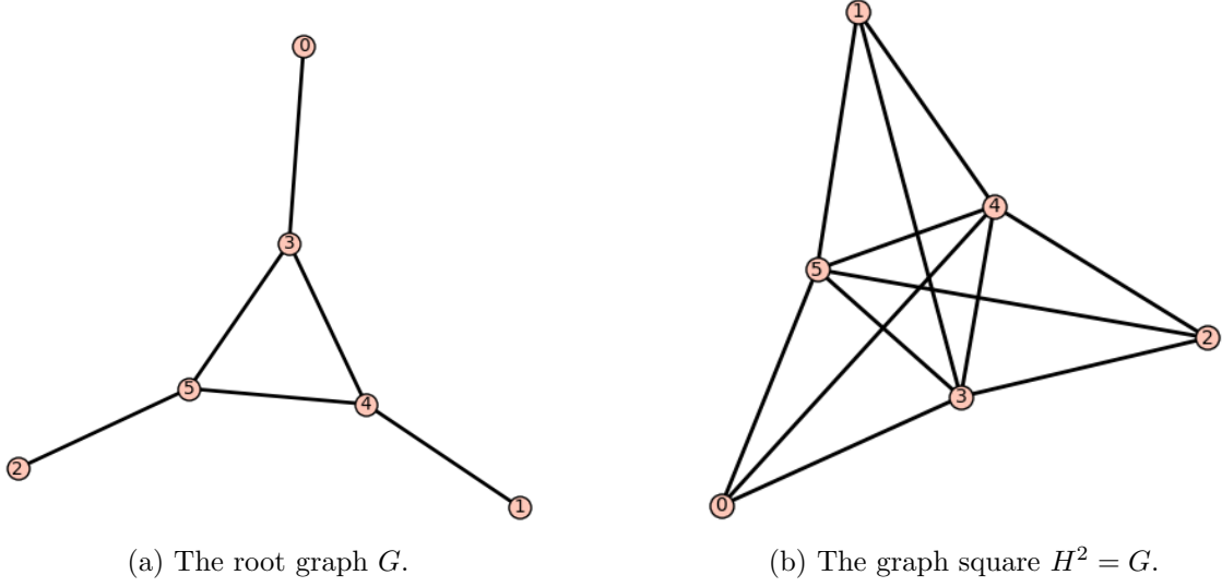
Figure 4.2: A six-vertex graph and its square. G only has one root that is unique up to isomorphism.
