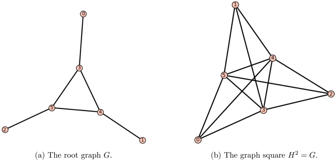
Figure 4.3: A six-vertex graph and its square. G only has one root that is unique up to isomorphism.
