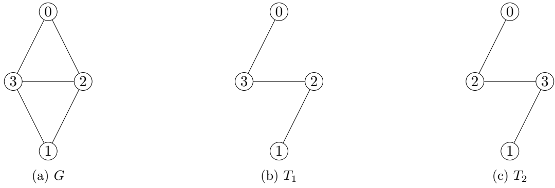
Figure 1.2: The graph G has two possible P_4 square roots, T_1 and T_2 . The two roots are isomorphic, differing only by the interchange of vertices 2 and 3.
