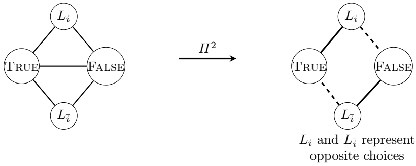
Figure 2.1: The gadgets illustrate how the structure of G_\phi constrains a square root H . The tail of x forces a root path and leaves a TRUE/FALSE choice. The clause tail similarly forces a root path and exposes the three literal vertices of the clause. Complementary literal vertices are constrained to represent opposite truth values and mirror the example in Figure 1.2 where (0, 1, 2, 3) = (L_i, L_{\bar{i}}, \text{FALSE}, \text{TRUE}) . Thus, the local structure of G_\phi encodes the truth assignment represented by a square root.
