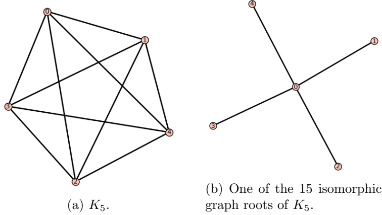
Figure 1.1: K_5 and one of its root, the star graph K_{1,4} .
