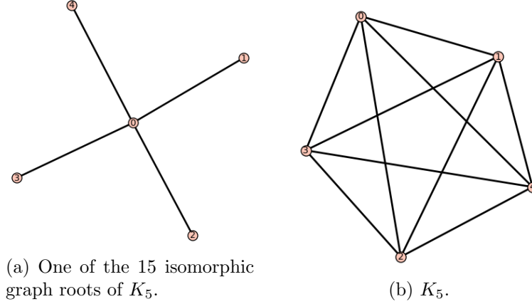
Figure 1.1: The star graph K_{1,4} and its square K_5 , which is a complete graph since every vertex in the root .
