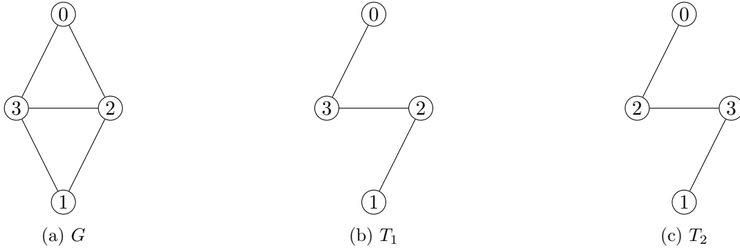
Figure 1.2: The graph G has two possible P_4 square roots that are trees, T_1 and T_2 . The two roots are isomorphic, differing only by the interchange of vertices 2 and 3.
