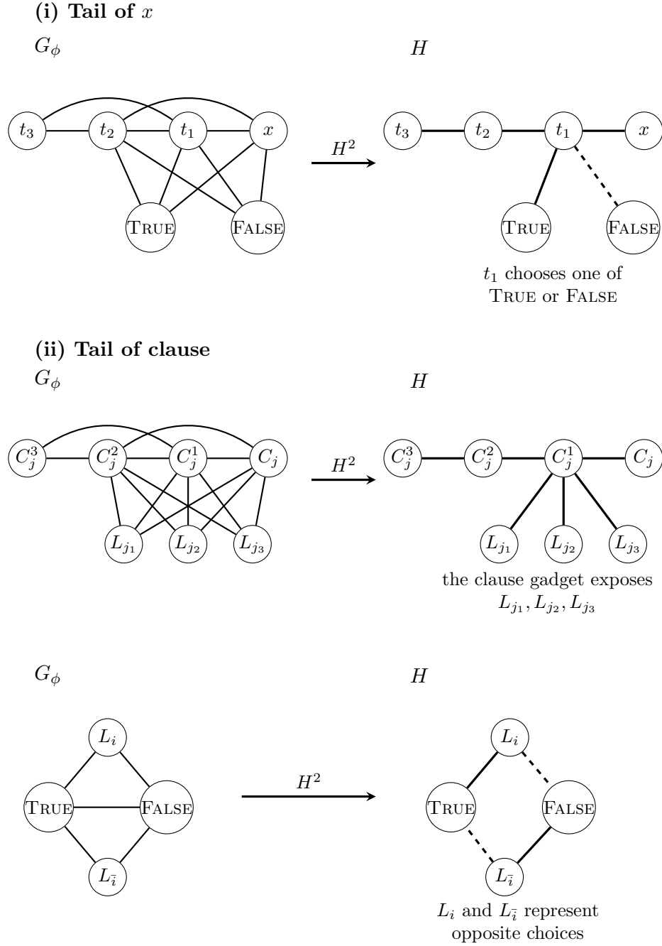
Figure 2.1: The gadgets illustrate how the structure of G_\phi constrains a square root H . The tail of x forces a root path and leaves a TRUE/FALSE choice. The clause tail similarly forces a root path and exposes the three literal vertices of the clause. Complementary literal vertices are constrained to represent opposite truth values. Thus, the local structure of G_\phi encodes the truth assignment represented by a square root.
