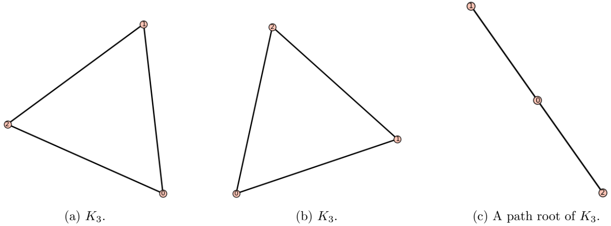
Figure 3.4: The graph K_3 and two of its square roots.
