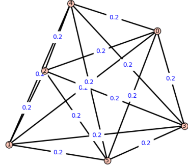
(a) \min \mathcal{LP}(G) result from K_6 input.
