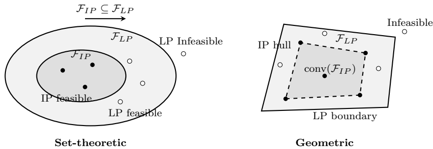
Figure 1.3: Set-theoretic and geometric relationships between an integer program and its linear relaxation.
