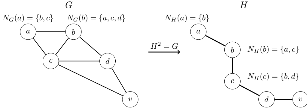
Figure 2.2: The forced local structure in the Tail Lemma. The square root H contains the path a - b - c - d . Consequently, ac, bd \in E_G as distance-two edges. For an external neighbour v of c , the Tail Lemma gives dv \in E_H , and hence dv \in E_G .
