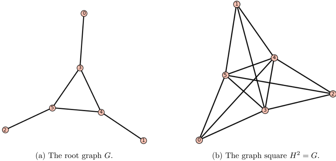
Figure 4.2: A six-vertex graph and its square. G only has one root, although there are different relabellings.
