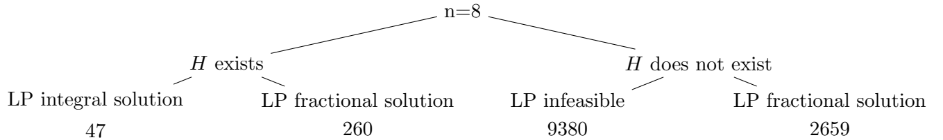
Figure 3.1: LP outcomes for n = 8 vertices on the base linear program.
