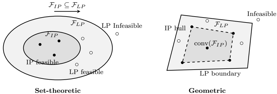
Figure 1.3: Set-theoretic and geometric relationships between an integer program and its linear relaxation.
