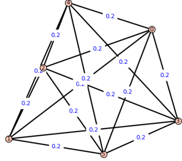
(b) \min \mathcal{LP}(G) result from K_6 input.
