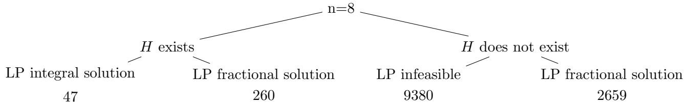
Figure 3.1: LP outcomes for n = 8 vertices using \mathcal{LP}(G) .
