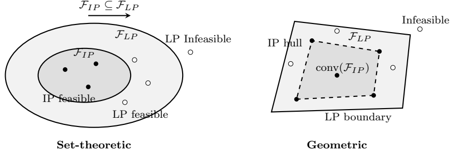
Figure 3.1: Set-theoretic and geometric relationships between an integer program and its linear relaxation.
