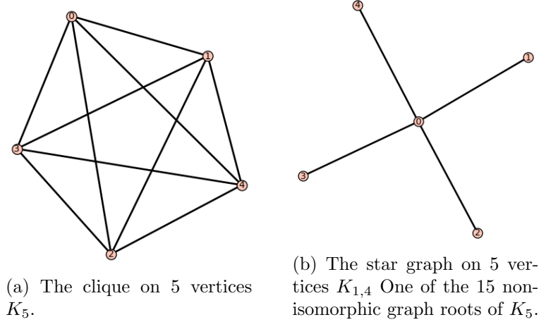
Figure 1.1: K_5 and two of its 15 non-isomorphic graph roots.
