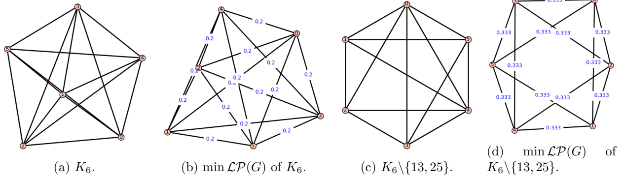
Figure 3.3: For the square graph K_6 , the result of \min \mathcal{LP}(G) is completely fractional with all edges having weight \frac{1}{5} . For the square graph K_6 \setminus \{13, 25\} , the result of \min \mathcal{LP}(G) is completely fractional with all edges having weight \frac{1}{3} .
