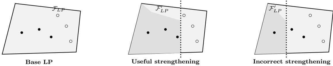
Figure 3.2: Strengthening the linear program with an additional constraint. Each panel shows the same feasible region and candidate solutions, with valid roots represented by filled black dots and invalid roots by unfilled white dots. The position of the additional constraint determines which solutions remain feasible. A suitable constraint eliminates fractional solutions while retaining all valid integer solutions, whereas an overly restrictive constraint also excludes valid integer solutions.
