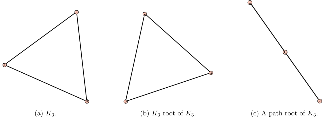
Figure 3.4: The graph K_3 and two of its square roots. Notice that there are multiple possible isomorphic P_3 roots.
