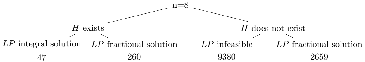
Figure 3.1: LP outcomes for n = 8 vertices using \mathcal{LP}(G) .
