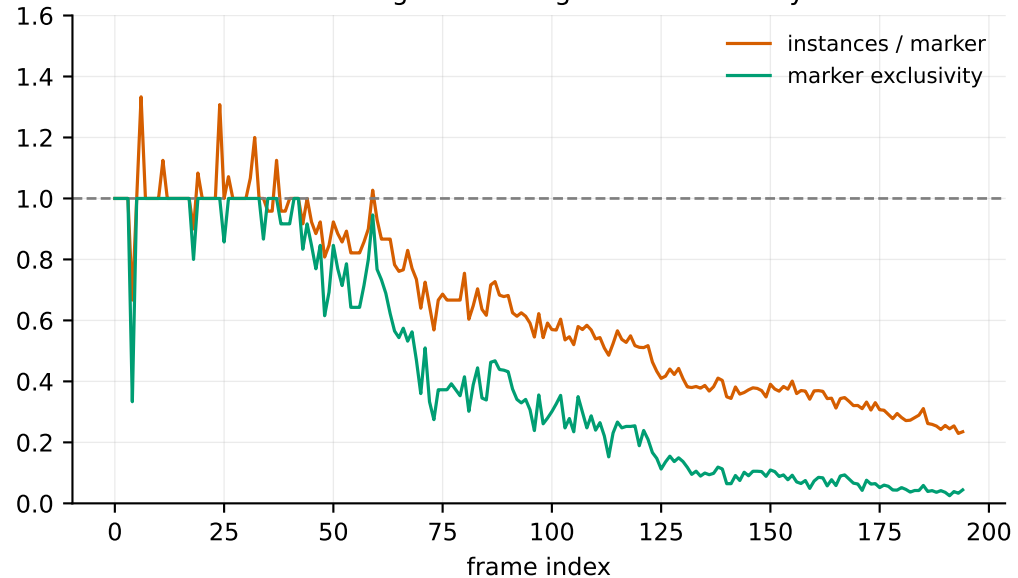
Under-segmentation grows with density
