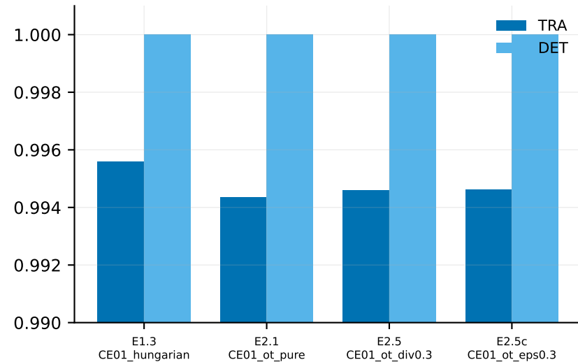
official CTC metrics
