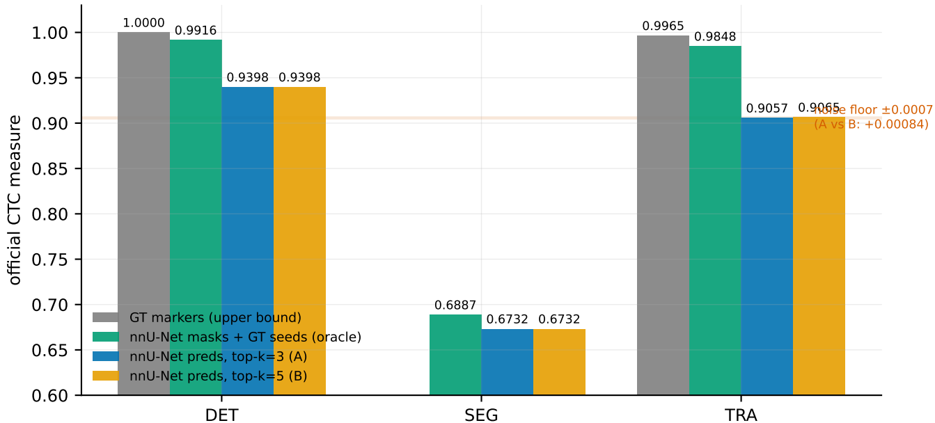
Detection source matters more than the tracking tweak (Fluo-N3DH-CE seq01)
