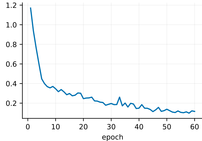
train loss
