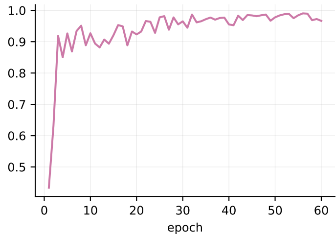
validation accuracy
