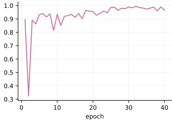
validation accuracy
