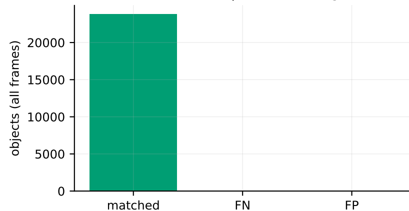
detection outcome | IDsw=353 frag=1454
