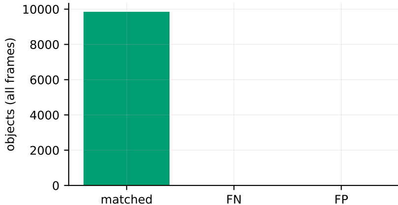
detection outcome | IDsw=7735 frag=6643
