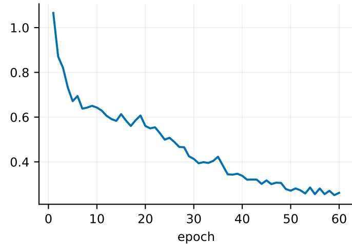
train loss
