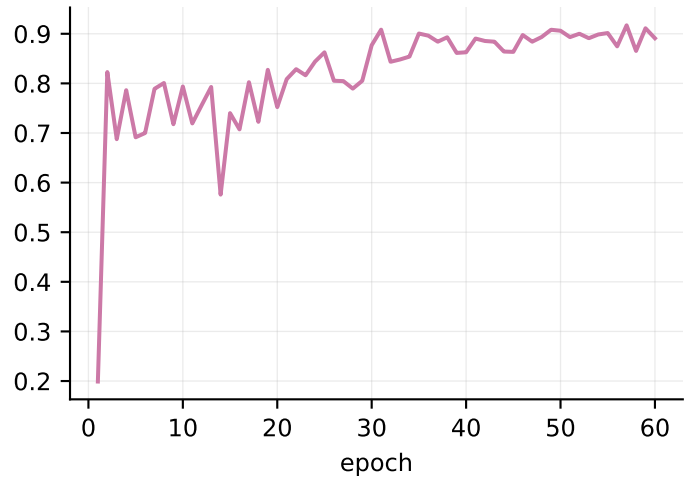
validation accuracy
