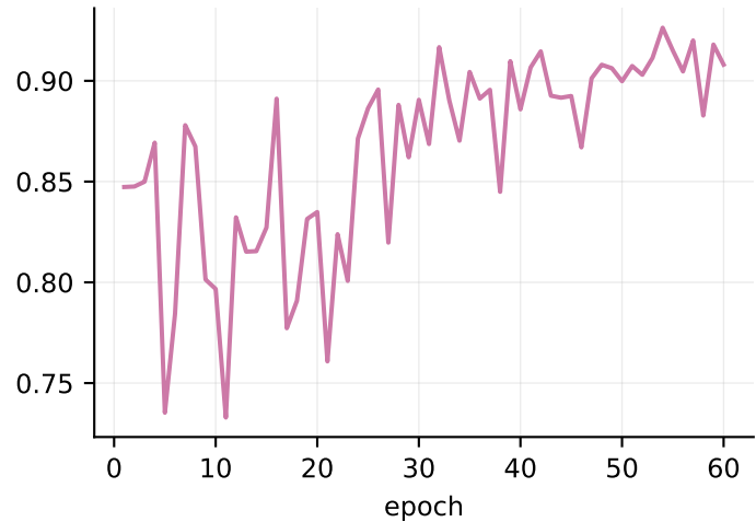
validation accuracy
