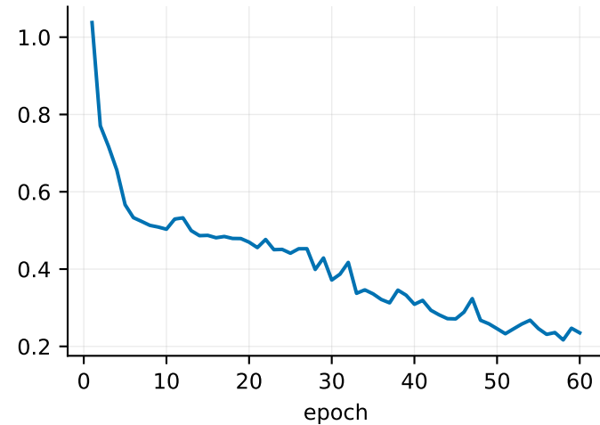
train loss
