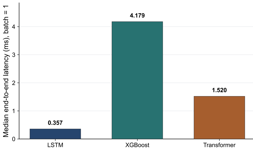
Figure 17: Median end-to-end batch-1 inference latency for the models compared in the source domain.
