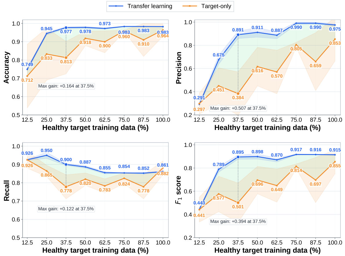
Figure 15: Fault detection performance on the fault-injected target test set D_{tgt}^{test-fault} under different proportions of healthy target training data. Curves show the mean and shaded bands show one sample standard deviation over five independent seeds.
