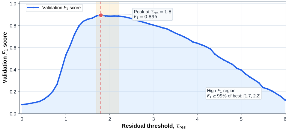
Figure 14: F1-score versus residual threshold on the fault-injected source validation set \mathcal{D}_{\text{src}}^{\text{val-fault}} ; the selected operating point is explicitly identified.
