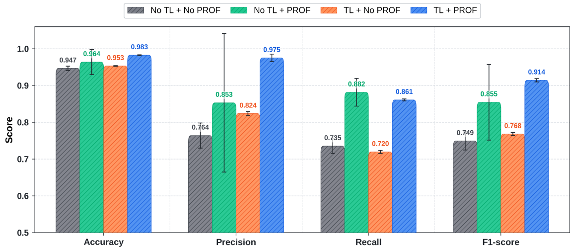
Figure 16: Fault-detection performance in the controlled TLxPROF ablation. Bars and error bars denote the five-seed mean and sample standard deviation.
