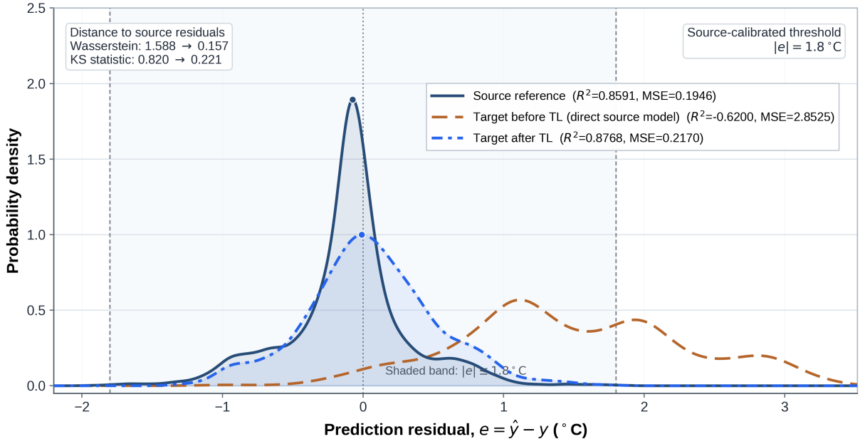
Figure 13: Controlled residual-density comparison for the original transfer experiment underlying Fig. 12. The solid blue curve shows source-domain residuals; the orange dashed curve shows the baseline obtained by applying the source-trained LSTM directly to the target test set; and the blue dash-dotted curve shows target-domain residuals after transfer learning. Both target curves use the identical 1,521 test windows. The vertical dashed lines indicate the source-calibrated decision boundary |e| = 1.8^\circ\text{C} .
