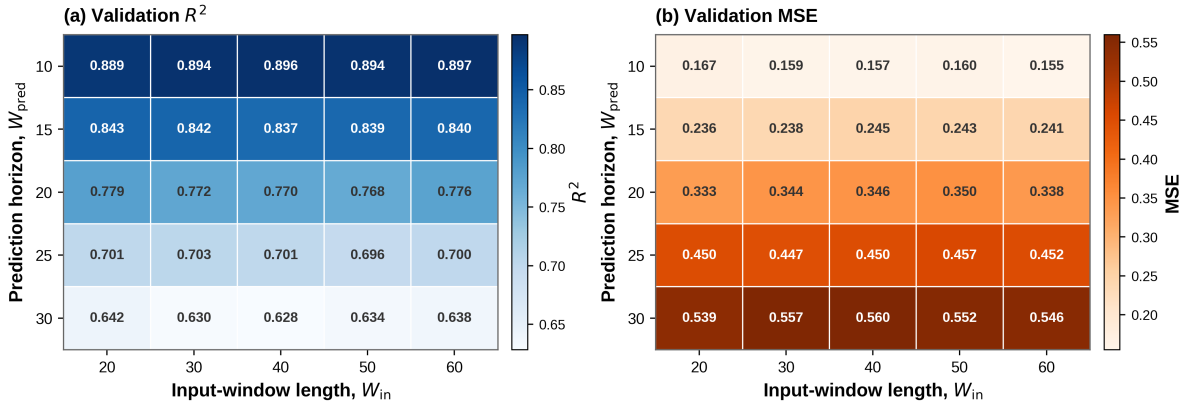
Figure 10: Sensitivity of source-domain validation performance to input-window length under different prediction horizons: (a) R^2 and (b) MSE. The outlined point denotes the retained W_{in} = 30 , W_{pred} = 10 setting.
