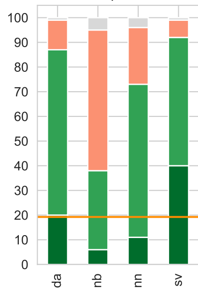
LOO, p = 0.1
