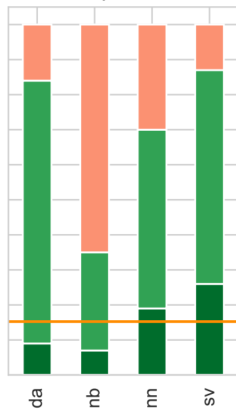
IG, p = 0.6
