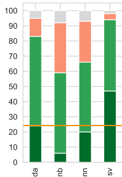
IG, p = 0.1
