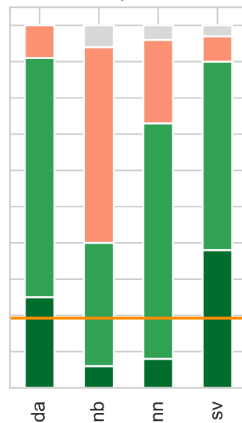
LIME, p = 0.1
