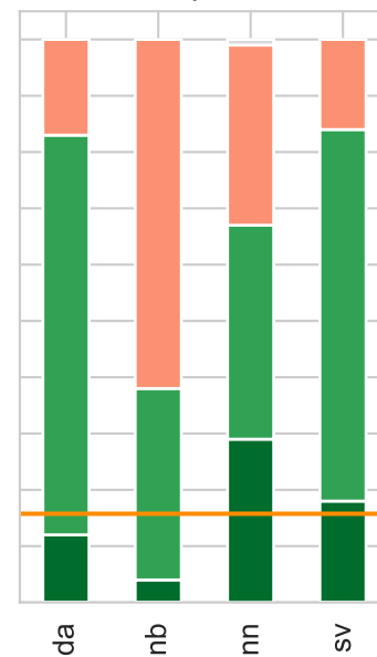
LIME, p = 0.6
