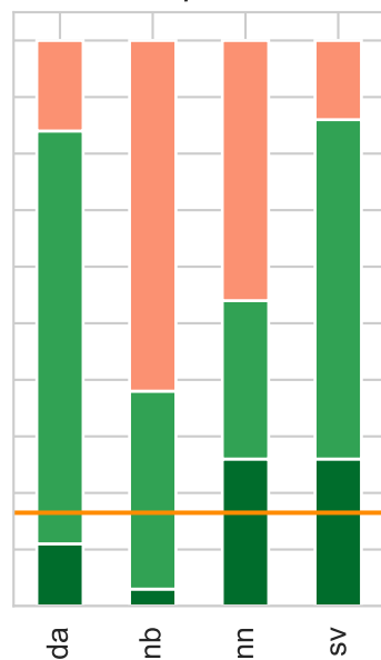
LOO, p = 0.6
