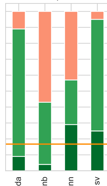
SHAP, p = 0.6
