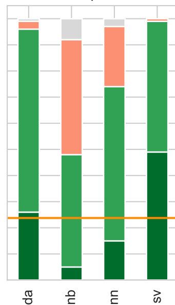
SHAP, p = 0.1
