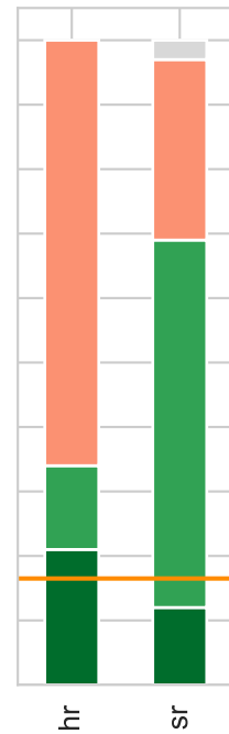
LOO, p = 0.6
