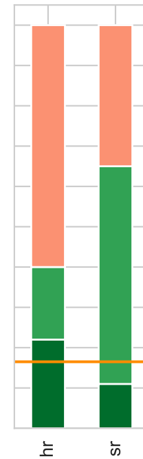
SHAP, p = 0.6
