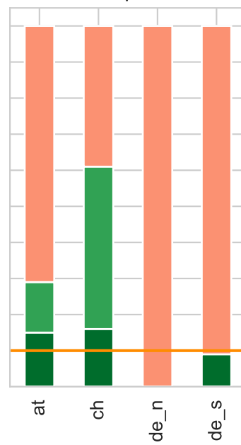
SHAP, p = 0.1
