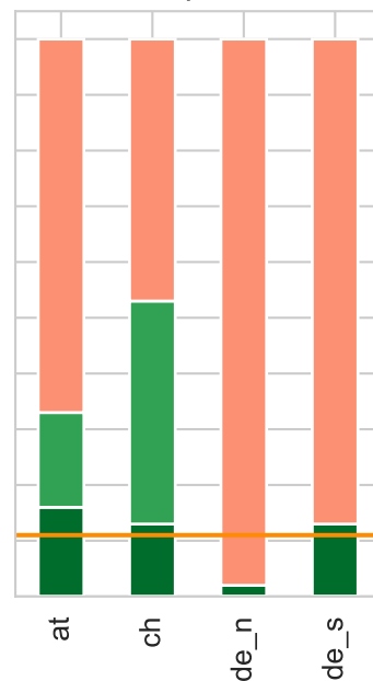
LIME, p = 0.1
