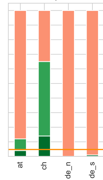
SHAP, p = 0.6
