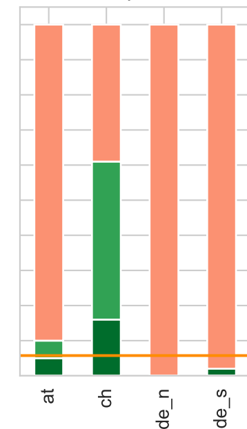
LIME, p = 0.6
