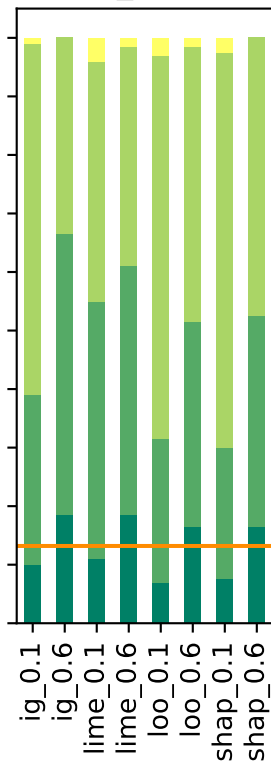
bcms_setimes
