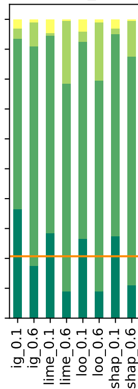
estonian_voro
