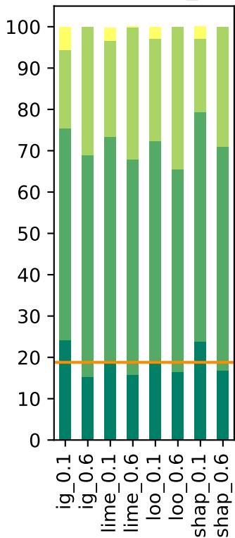
scandinavian_slide
