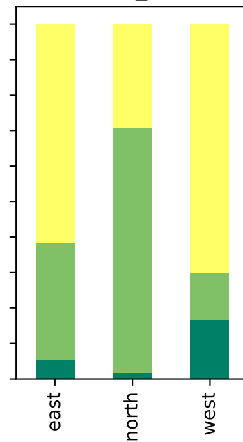
shap_0.1
