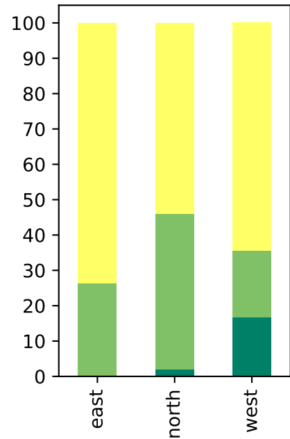
loo_0.1
