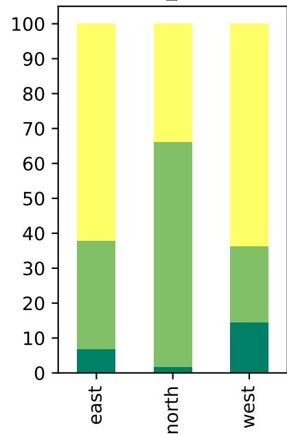
loo_0.1
