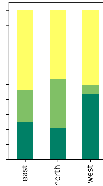
shap_0.6
