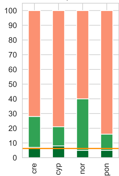
LOO, p = 0.1
