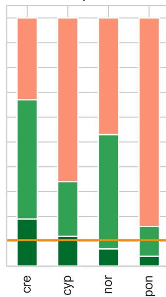
LIME, p = 0.1
