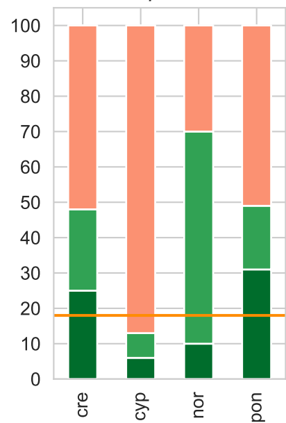
IG, p = 0.1
