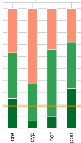
IG, p = 0.6
