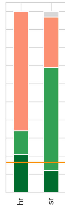
LOO, p = 0.6
