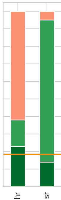
IG, p = 0.6
