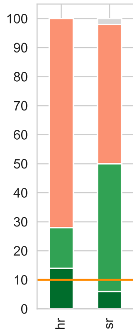
IG, p = 0.1
