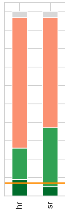
LOO, p = 0.1
