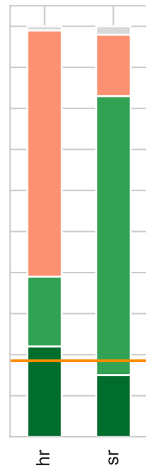
LIME, p = 0.6
