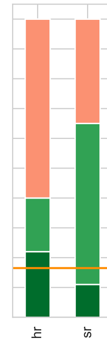
SHAP, p = 0.6
