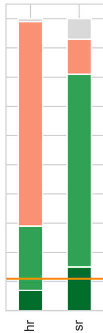
LIME, p = 0.1
