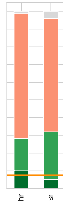
SHAP, p = 0.1
