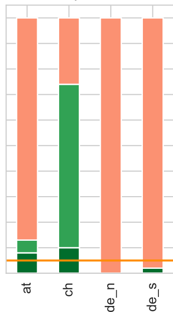
IG, p = 0.6
