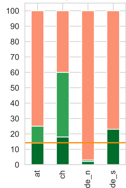
IG, p = 0.1
