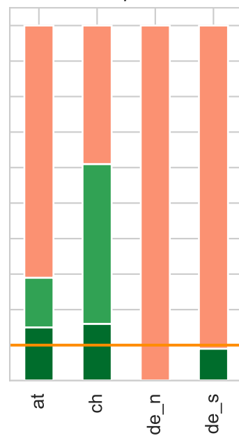
SHAP, p = 0.1
