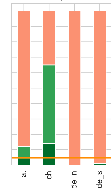
SHAP, p = 0.6
