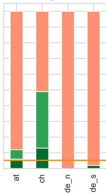
LOO, p = 0.6
