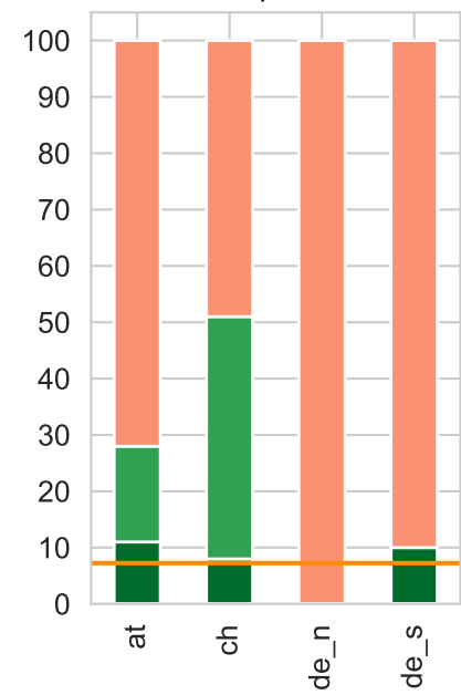
LOO, p = 0.1
