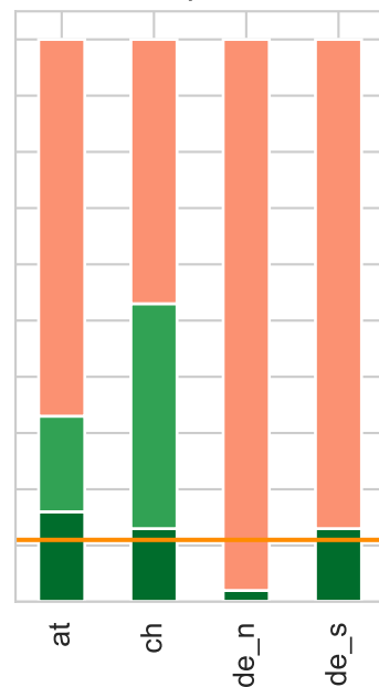
LIME, p = 0.1
