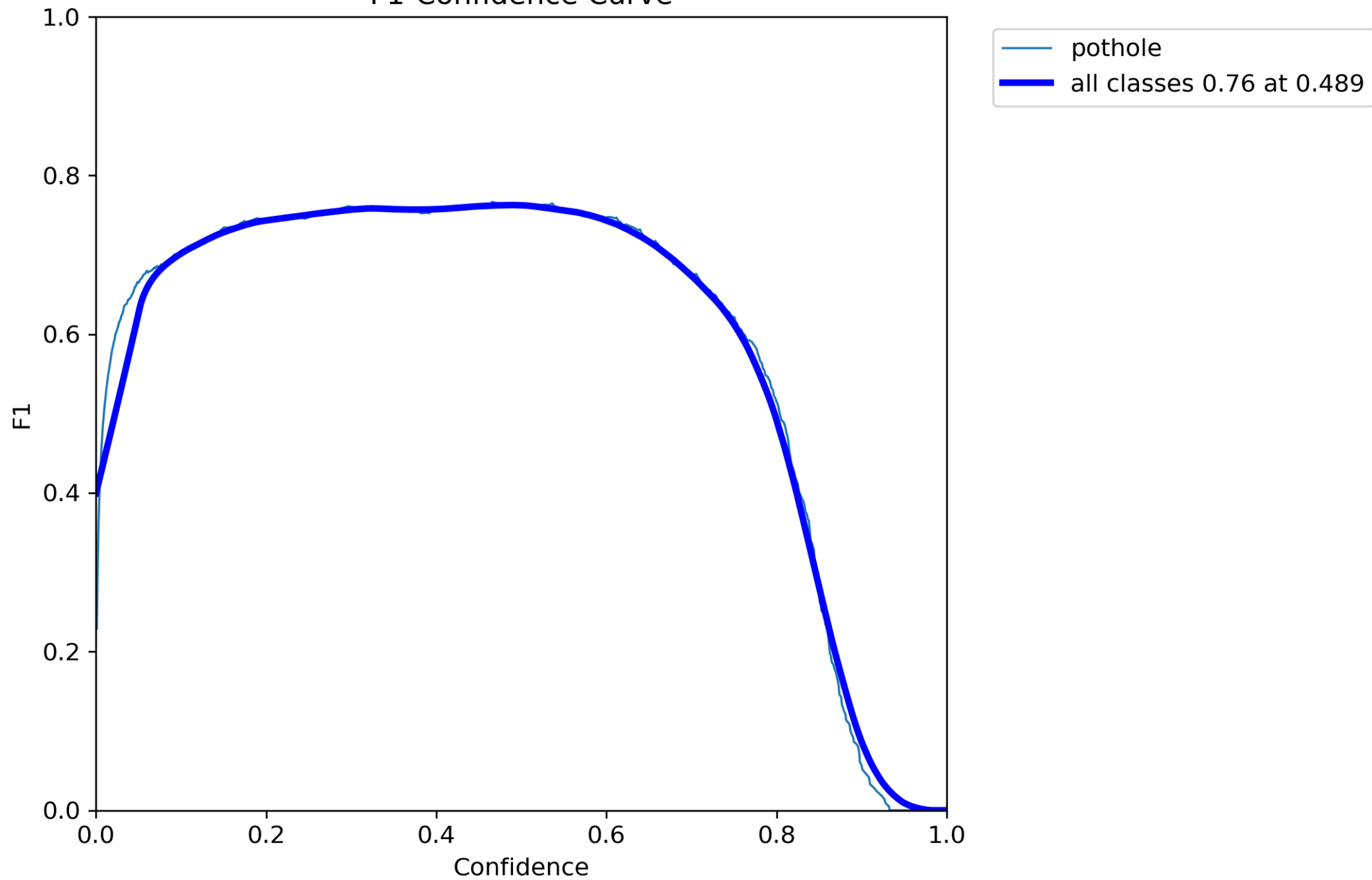
F1-Confidence Curve
