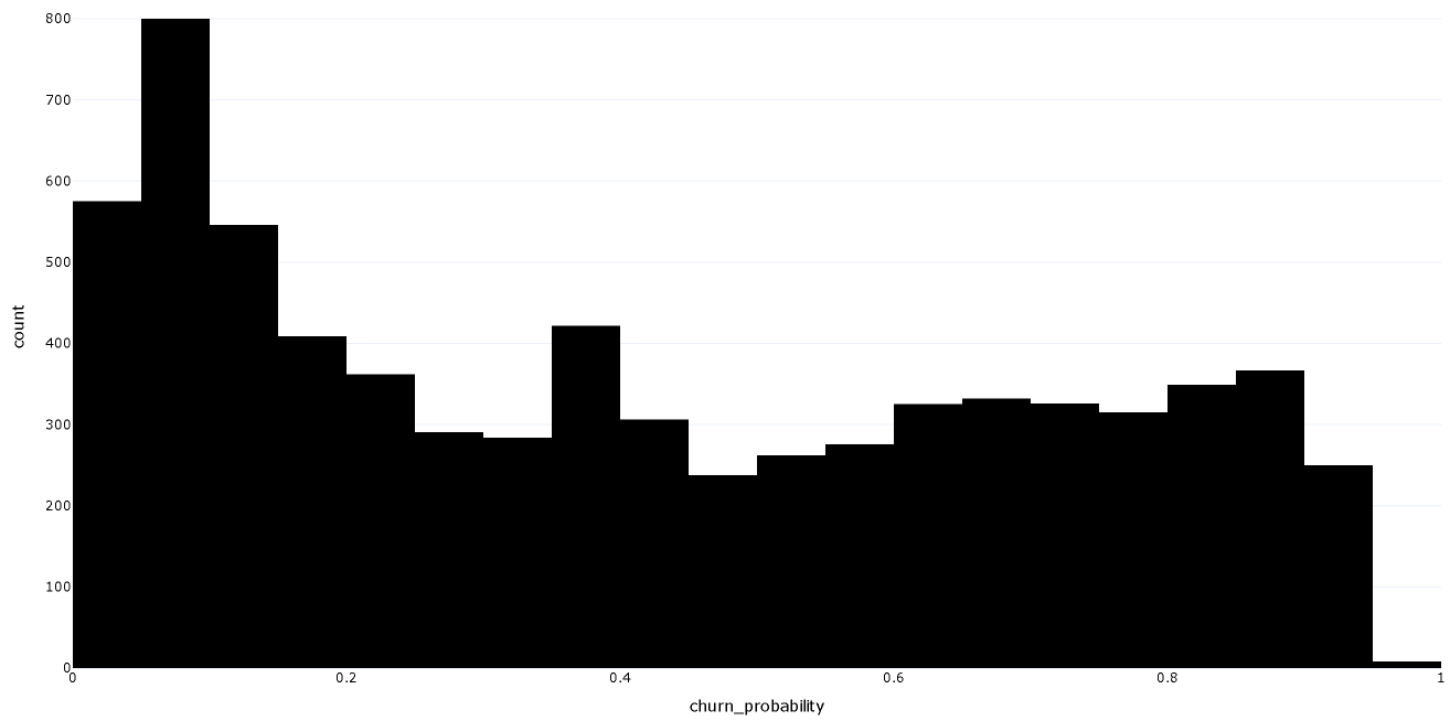
Churn Probability Distribution
