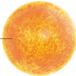
Yellow main sequence
