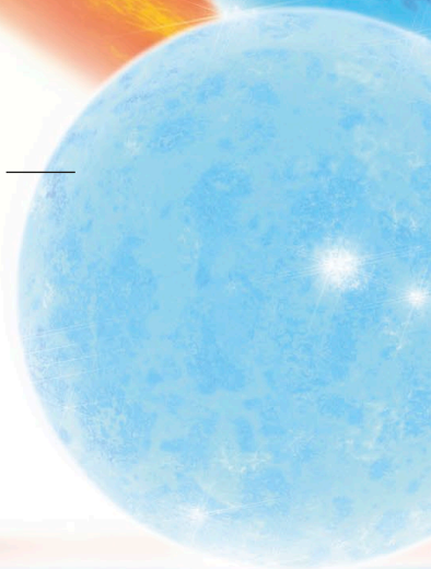
Blue supergiant
