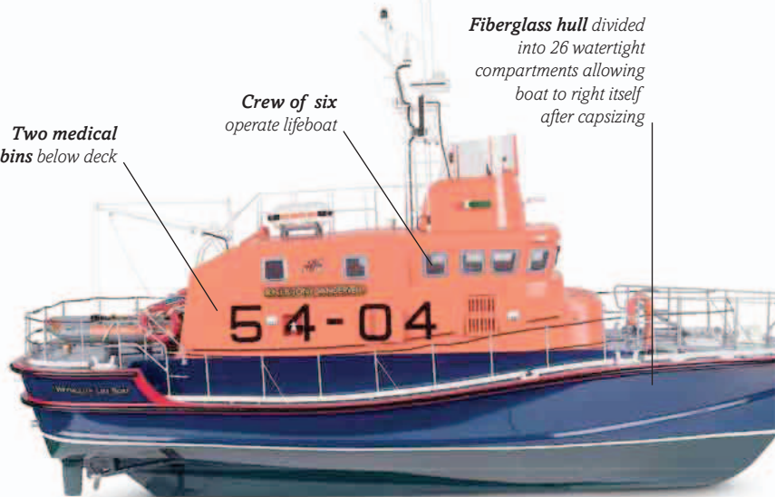
52 ft (16 m) long Arun class lifeboat UK 1970s–1990s
